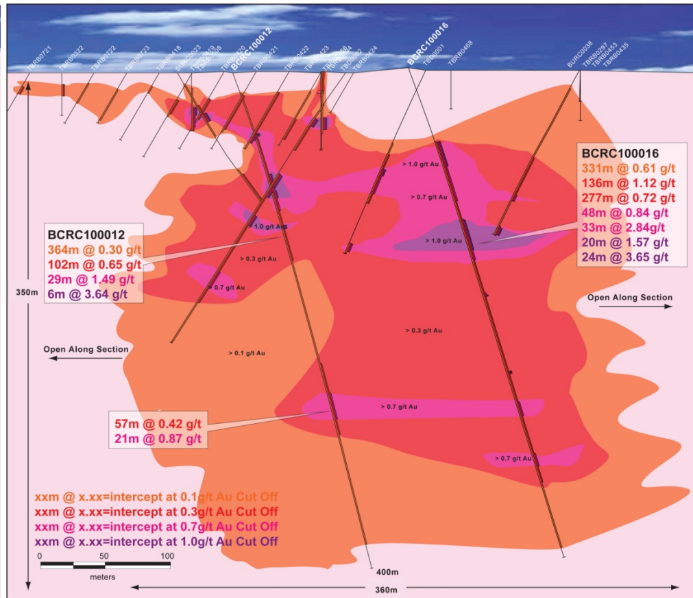
Cross-Section E
